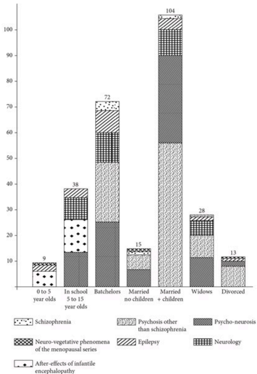
Graph 13 Diagnosis (women, 1959).
