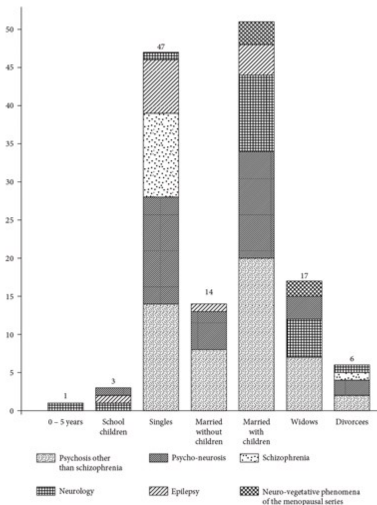
Graph 7 Diagnosis (women, 1958).
